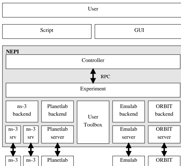
Figure 1: The Nepi architecture
