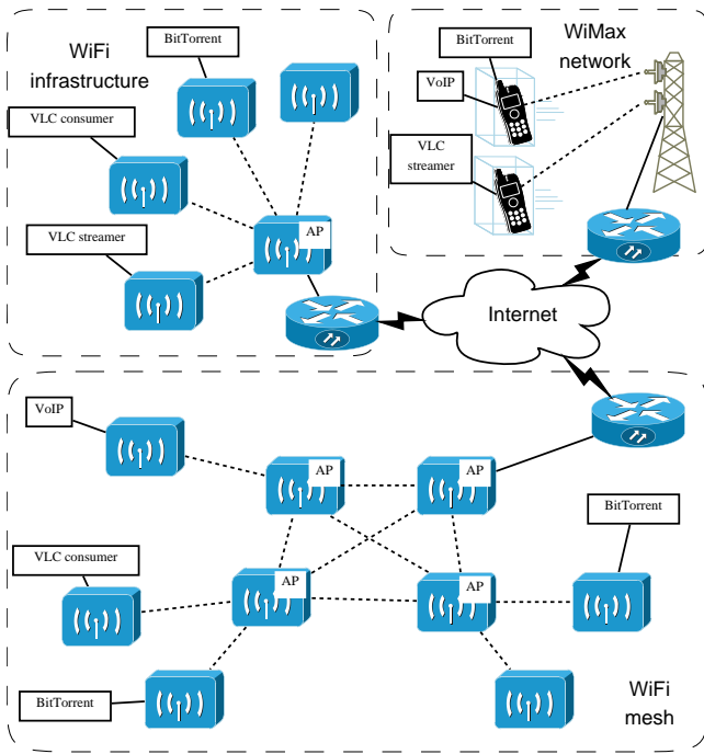
Figure 5: Conceptual diagram of a sample experiment
