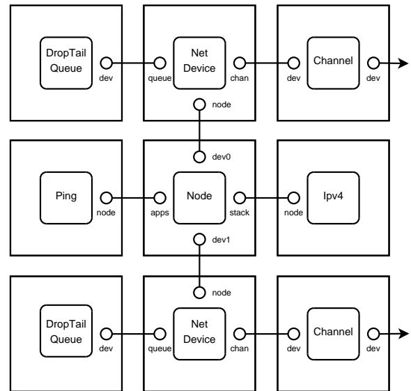
Figure 4: Description of a multihomed host in ns-3
