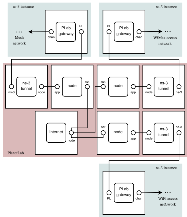
Figure 6: Partial representation of the experiment in Nepi
