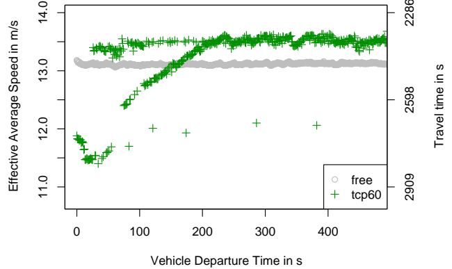
(b) 1000 vehicles on a 16×16 grid; lead vehicle stops for 240 s
