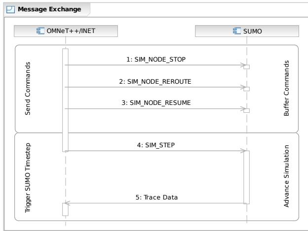
Figure 2: Messages exchanged between road traffic and network simulator communication modules.
