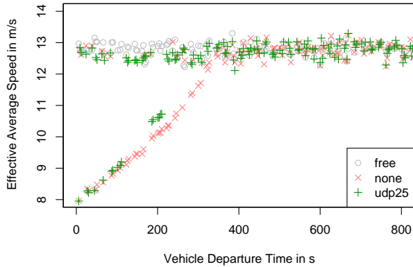
(a) Average speed ordered by time of departure
