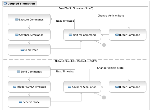
Figure 1: Overview of the coupled simulation framework. State machines of road traffic and network simulator communication modules.
