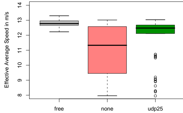
(b) Average speed grouped by scenario
