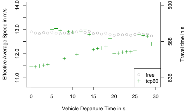
(a) 30 vehicles on a 5×5 grid; lead vehicle stops for 60 s
