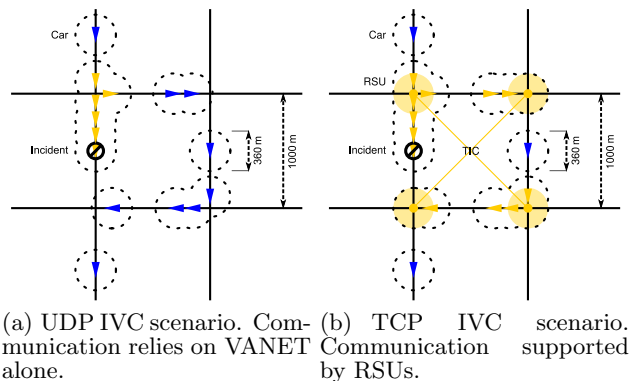
Figure 5: The two types of examined IVC scenarios.
