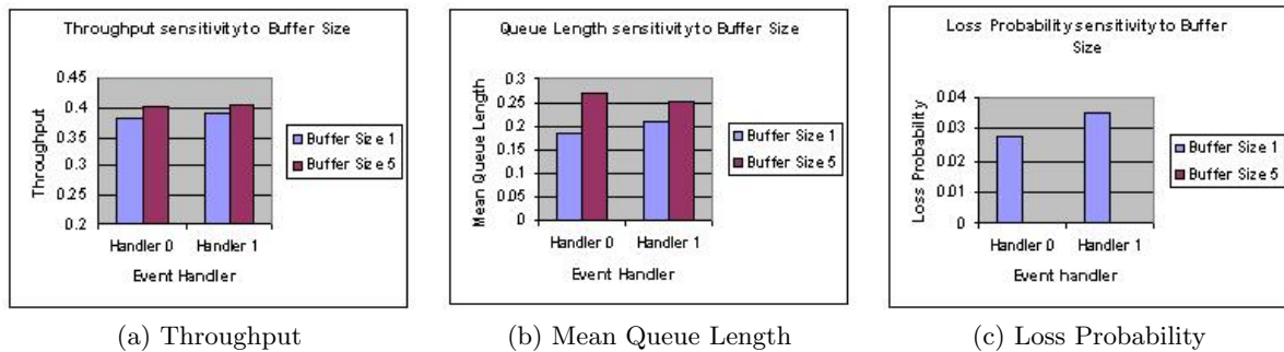
Figure 7: Effect of Maximum Buffer Size
