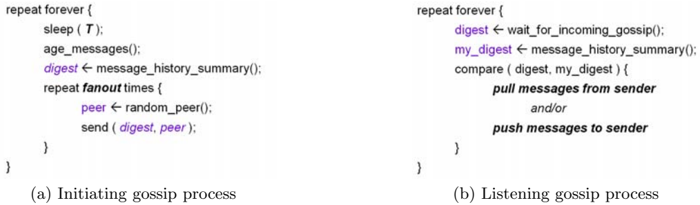
Figure 1: Skeleton Gossiping Psuedocode
